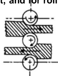
(b) Three high roll mill.
