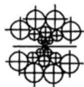
(e) Multi high roll mill.
