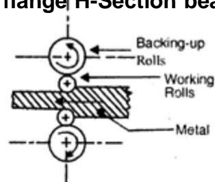
(c) Four high roll mill.
