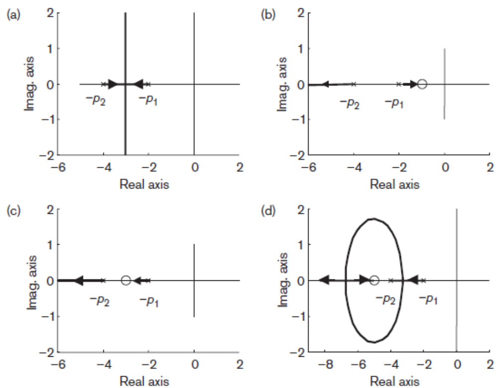
Figure 1 Effect of adding a zero to a second-order system root locus.
