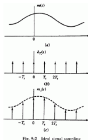
Fig. 5-2 Ideal signal sampling
