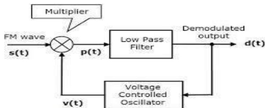
Foster Seeley FM Demodulator (Block diagram)
