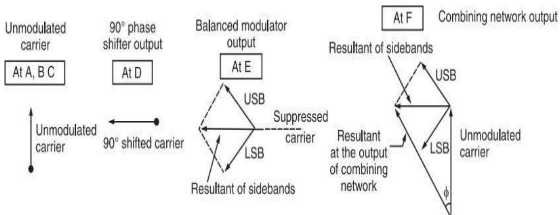
Fig.2: Phasors explaining the generation of PM
