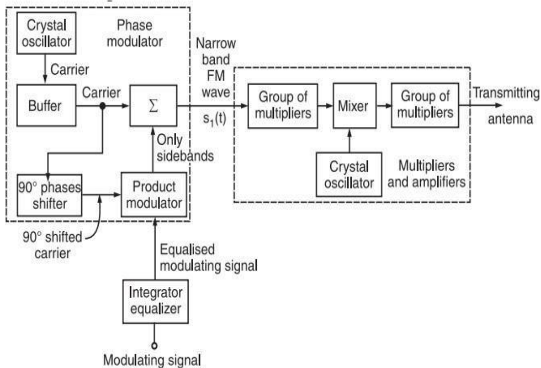
Fig.1 : Armstrong Method for FM Generation
