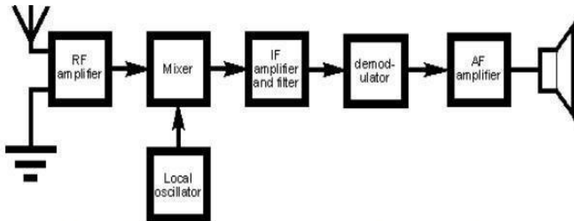
FIG 1.10 Block Diagram of a Basic Superheterodyne Radio Receiver
