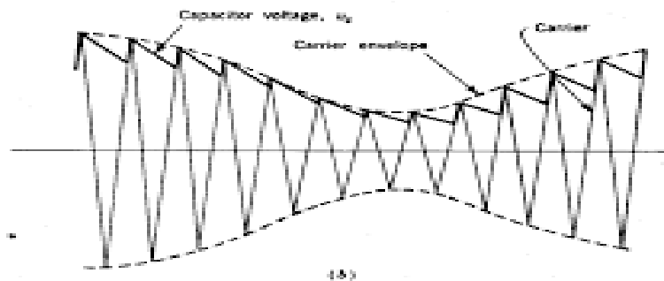
Figure 3.4-2 (a) A demodulator for an AM signal. (b) Input waveform and output voltage v_c across capacitor.
