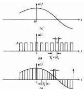
Natural Sampled Waveform
