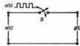
Functional Diagram of Natural Sampler
