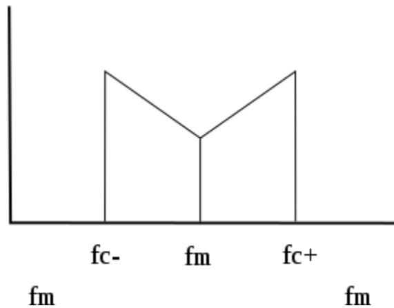
Spectrum plot of a DSB-SC signal:
