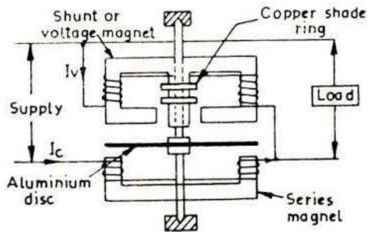
Induction type wattmeter
