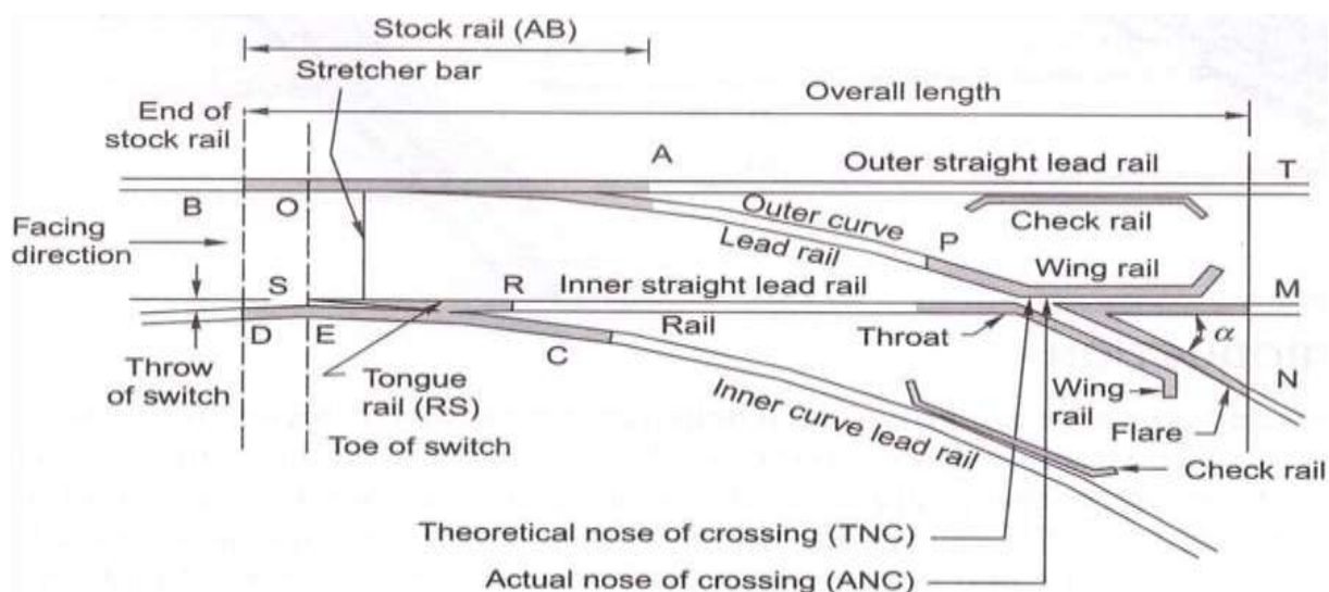
(Constituents of a turnout)
