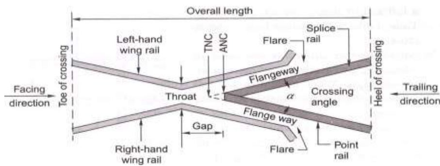
(Details of a crossing)
