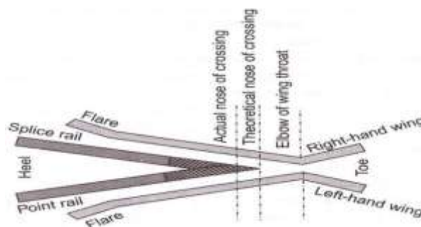
(Details of a crossing)
