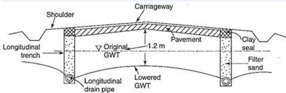
Fig. Lowering GWT in pervious soil by Subsurface drains
