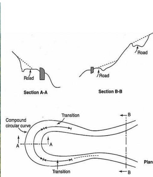
Schematic dig. of hair pin bend curve
