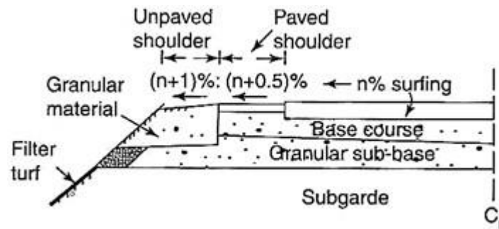
Fig. Shoulder Drainage
