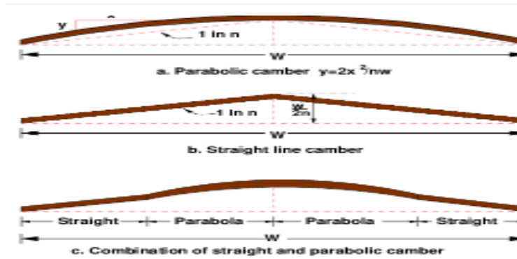
Figure : Different types of camber
