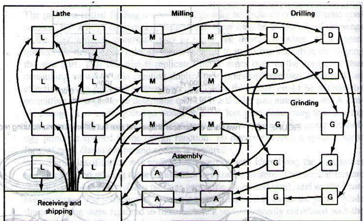
Process-type layout.
